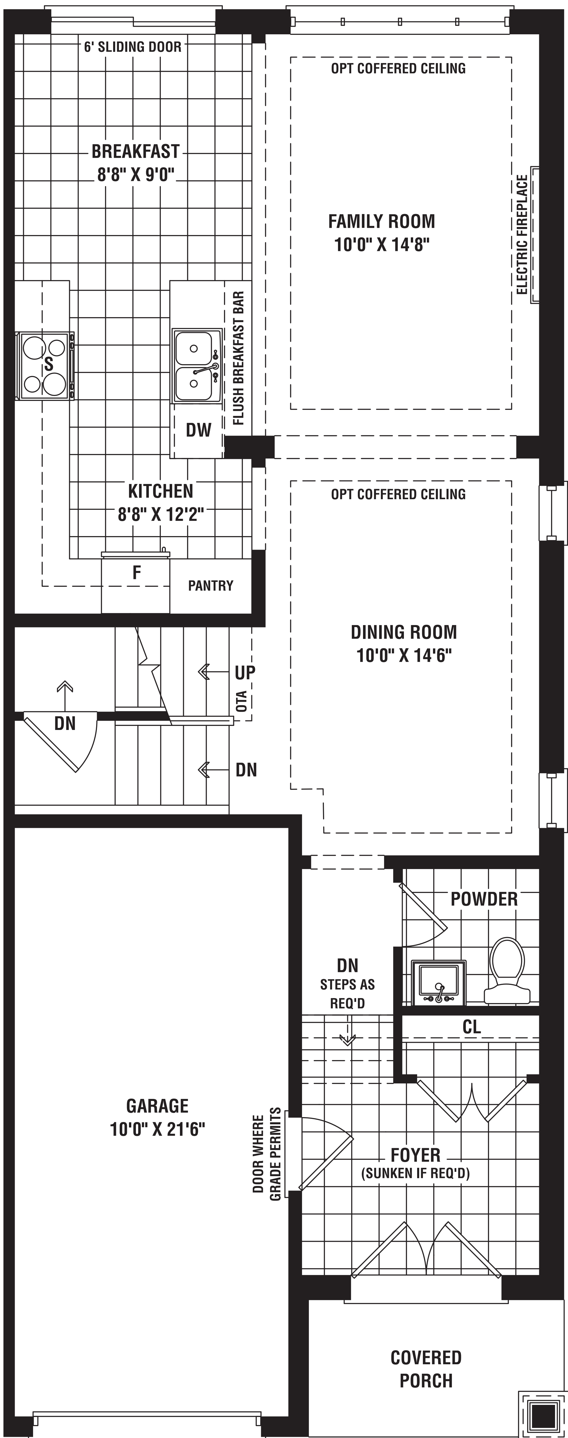
GROUND FLOOR ELEV. 'A'
